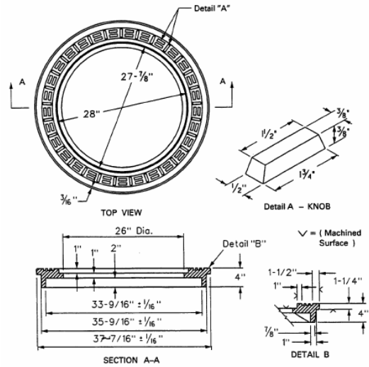
26" - 36" MH Ring
