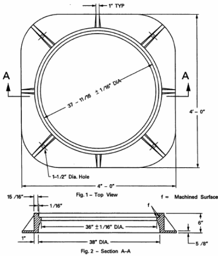
36" MH Frame
