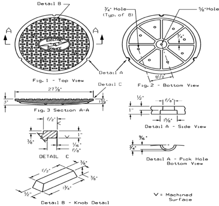
26" MH Cover
