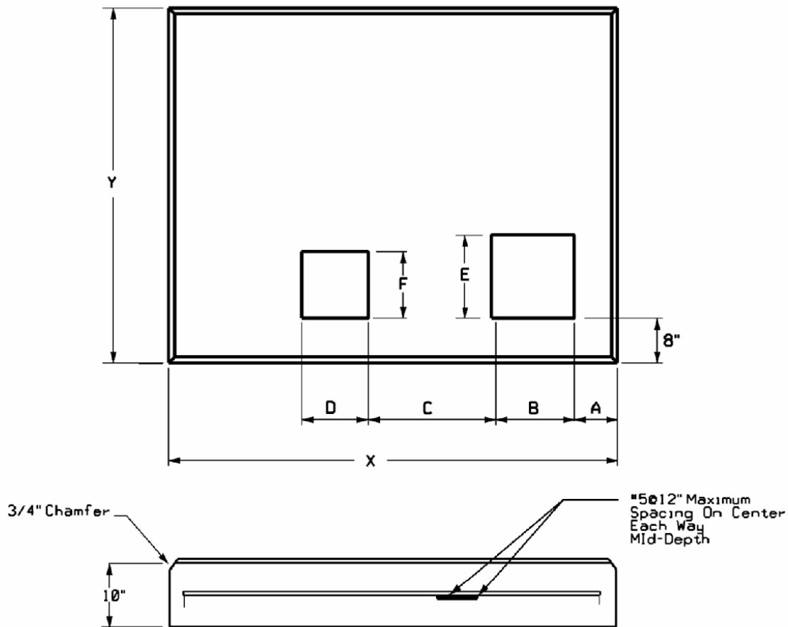
REBAR DIAGRAM
