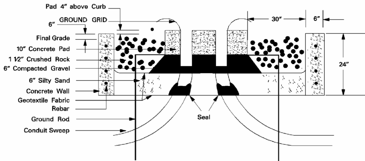
Typical Detail
