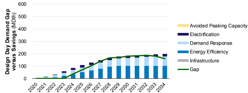
Figure A24: No Infrastructure – Low Demand Scenario
