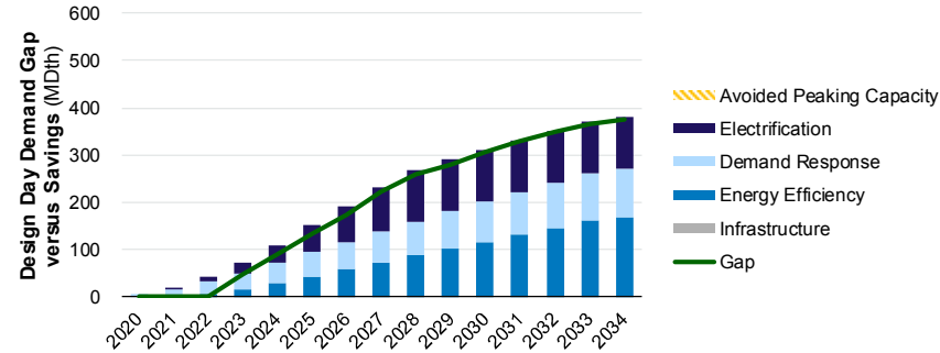
Figure A23: No Infrastructure – High Demand Scenario
