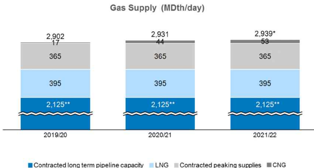
Figure 17: Summary of existing and near-term sources of Downstate NY gas supply
